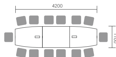
ST14 X2 TABLE 1400/1100/730 ST14S TABLE 1400/1100/730
